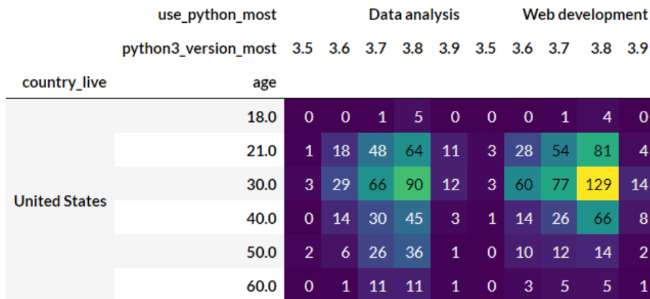
Figure 29.1: Jupyter showing a view of dataframe with a heatmap. This pulls attention to versions and ages that are most common.
