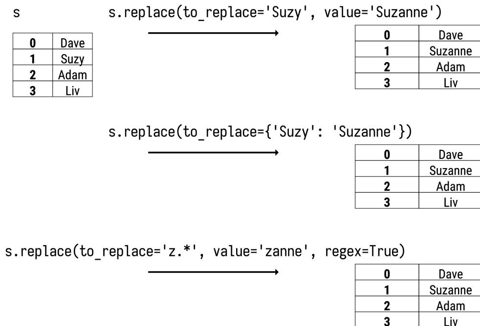
Figure 9.7: The .replace method illustrating different replacement mechanisms.
