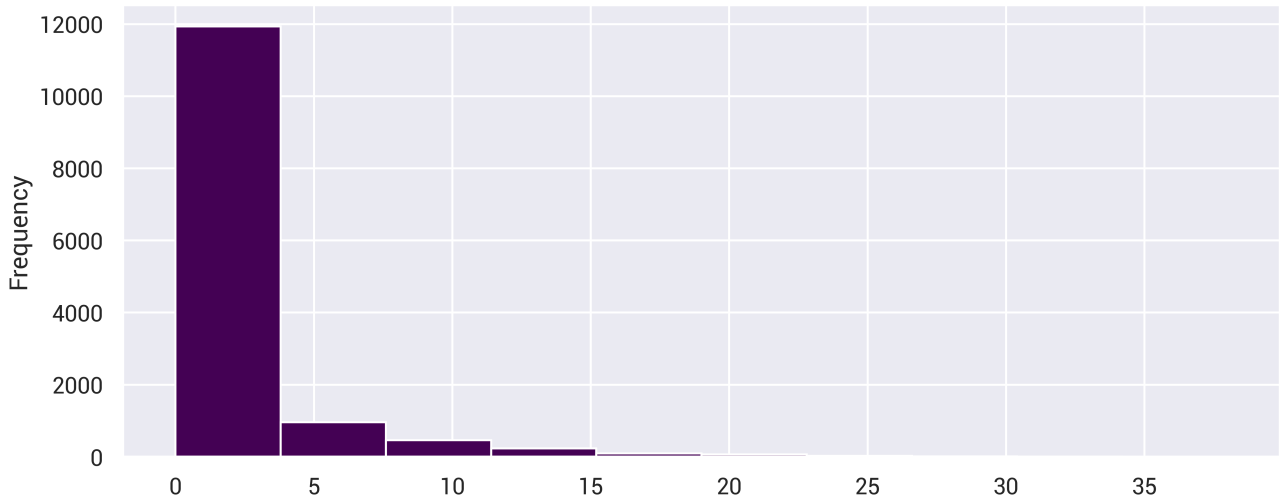
Figure 14.1: Basic histogram.
