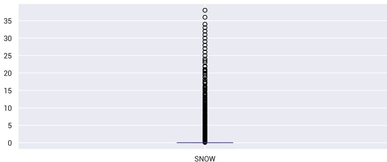
Figure 14.3: Basic boxplot.
