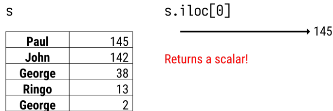
Figure 10.8: Indexing off of the .iloc attribute will return a scalar by location in the series.
