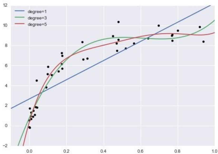
Figure 5-27. Three different polynomial models fit to a dataset
