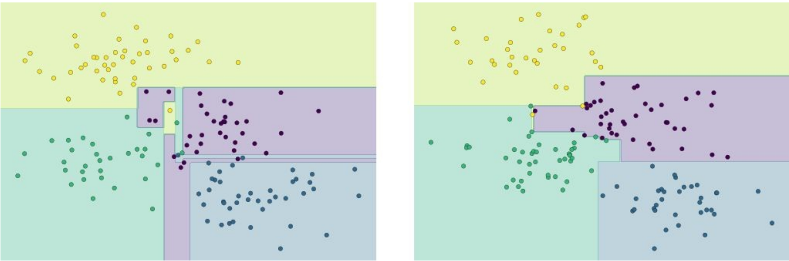
Figure 5-72. An example of two randomized decision trees
