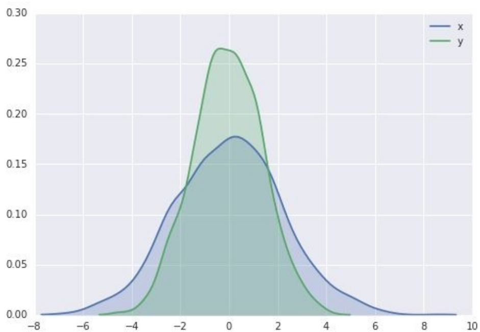
Figure 4-114. Kernel density estimates for visualizing distributions
