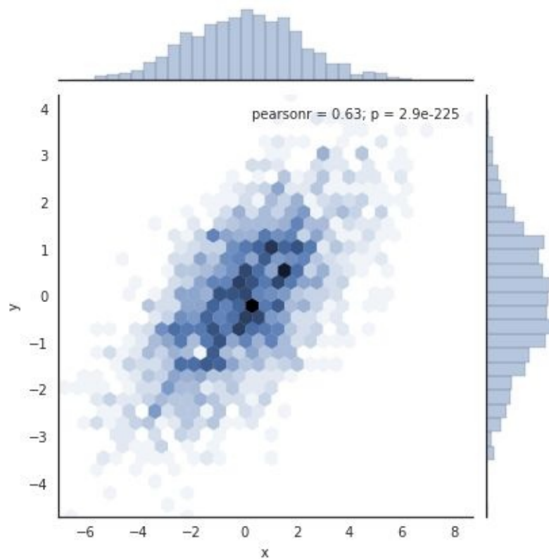
Figure 4-118. A joint distribution plot with a hexagonal bin representation
