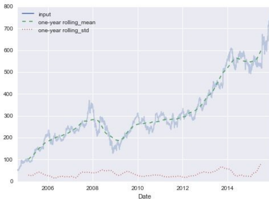
Figure 3-10. Rolling statistics on Google stock prices
