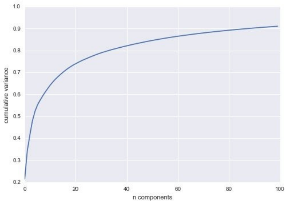
Figure 5-105. Cumulative variance from the PCA projection
