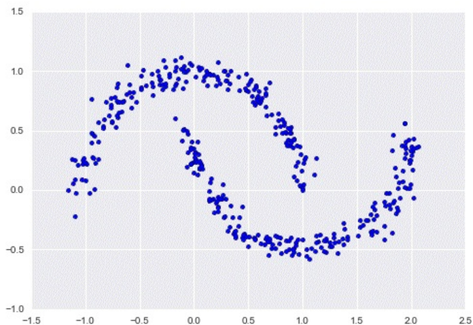
Figure 5-135. New data drawn from the 16-component GMM
