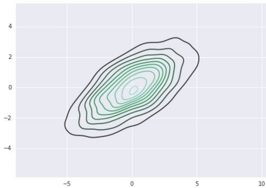
Figure 4-116. A two-dimensional kernel density plot
