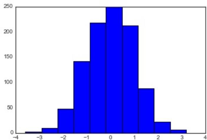
Figure 4-35. A simple histogram
