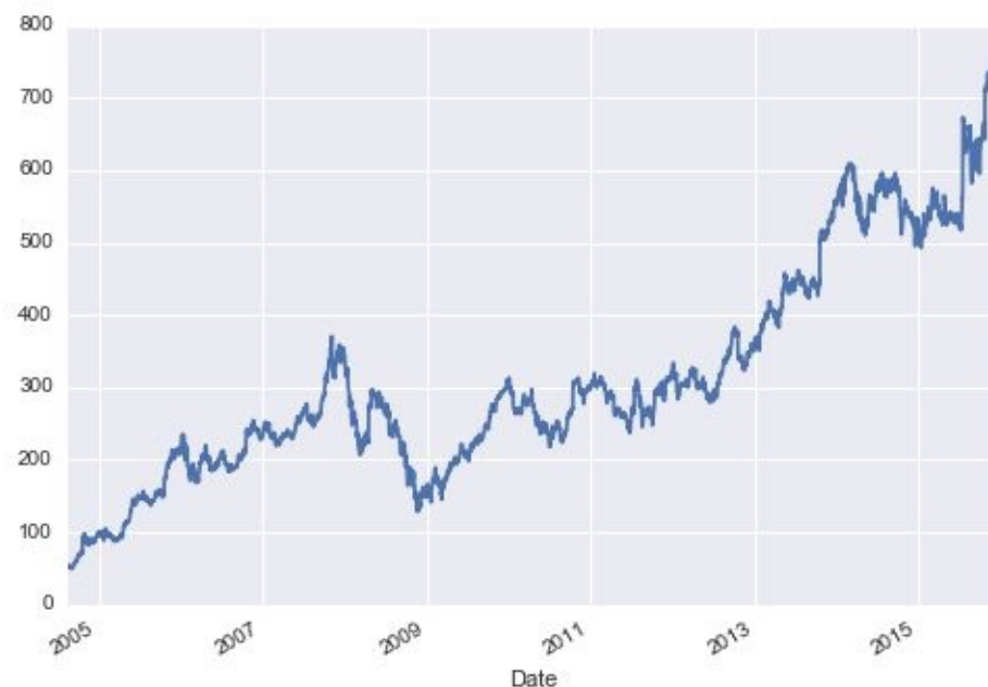
Figure 3-5. Google's closing stock price over time
