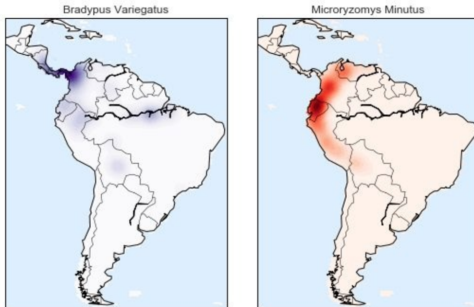
Figure 5-147. A kernel density representation of the species distributions
