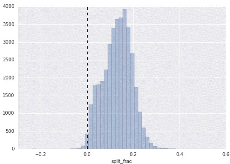
Figure 4-127. The distribution of split fractions; 0.0 indicates a runner who completed the first and second halves in identical times
