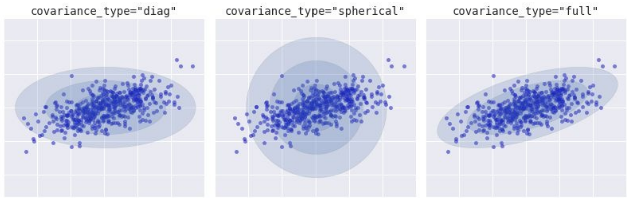
Figure 5-131. Visualization of GMM covariance types
