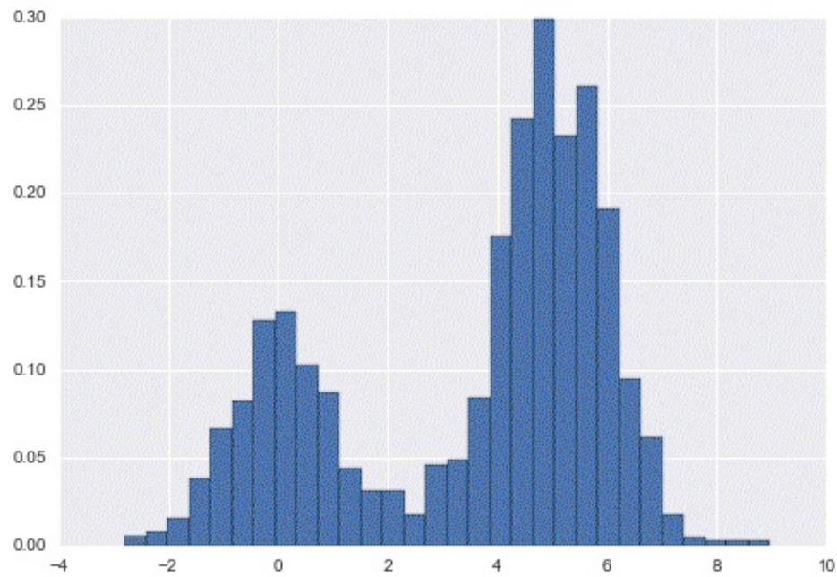
Figure 5-140. Data drawn from a combination of normal distributions
