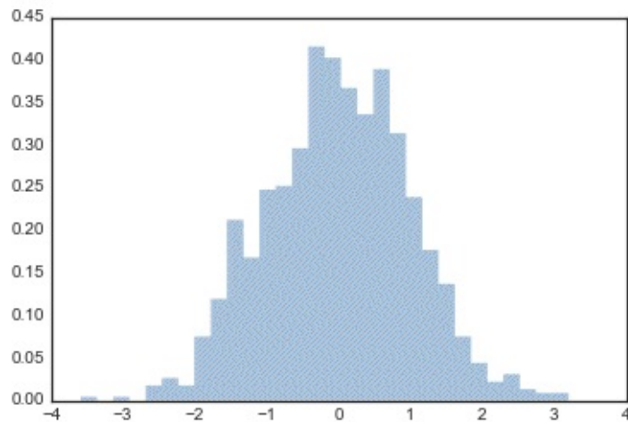
Figure 4-36. A customized histogram
