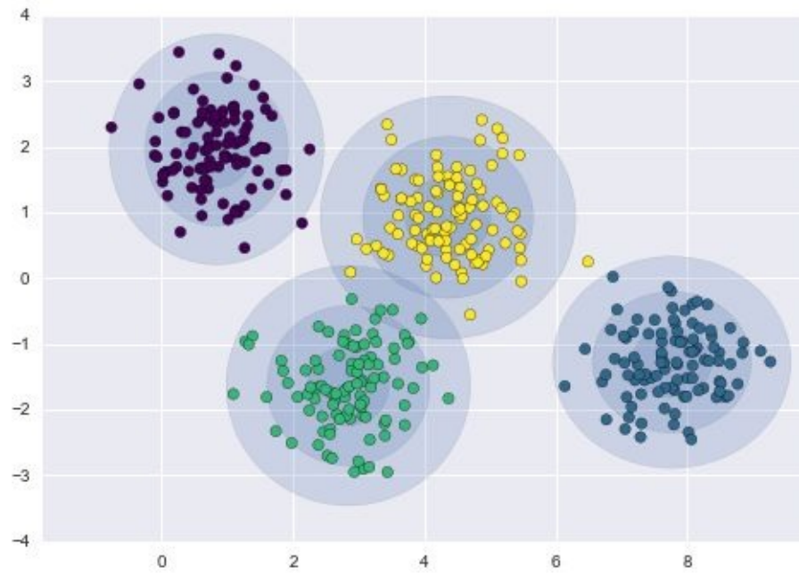
Figure 5-129. Representation of the four-component GMM in the presence of circular clusters
