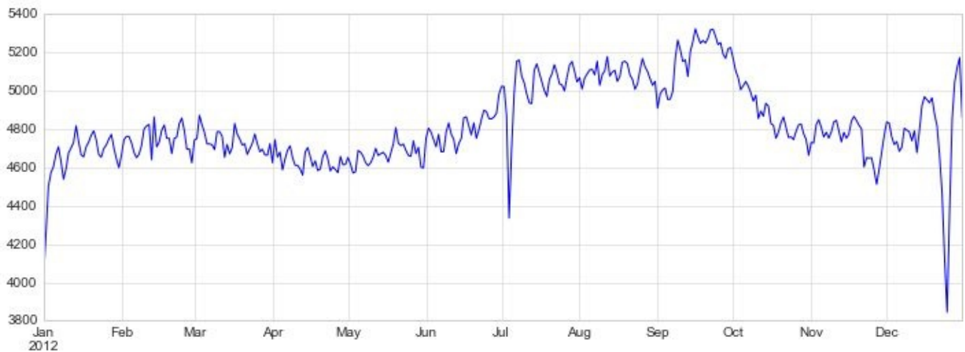
Figure 4-67. Average daily births by date
