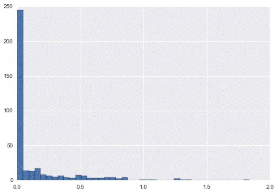
Figure 2-6. Histogram of 2014 rainfall in Seattle
