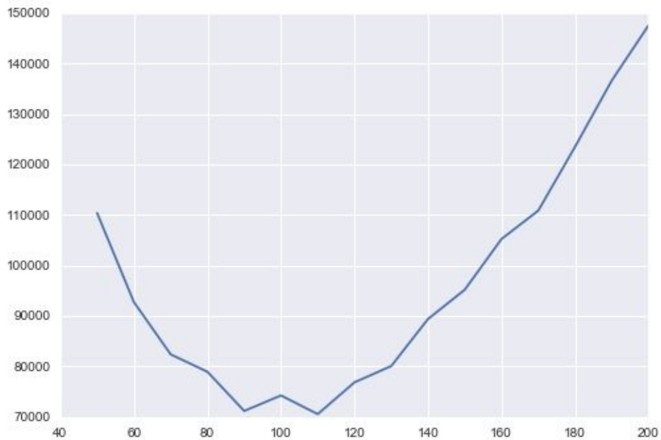
Figure 5-138. AIC curve for choosing the appropriate number of GMM components
