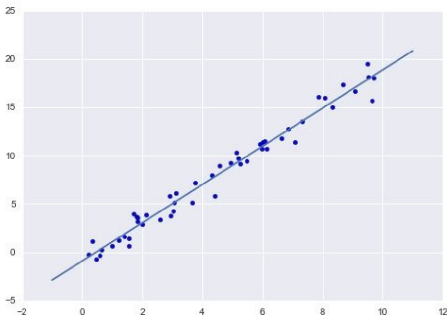
Figure 5-15. A simple linear regression fit to the data
