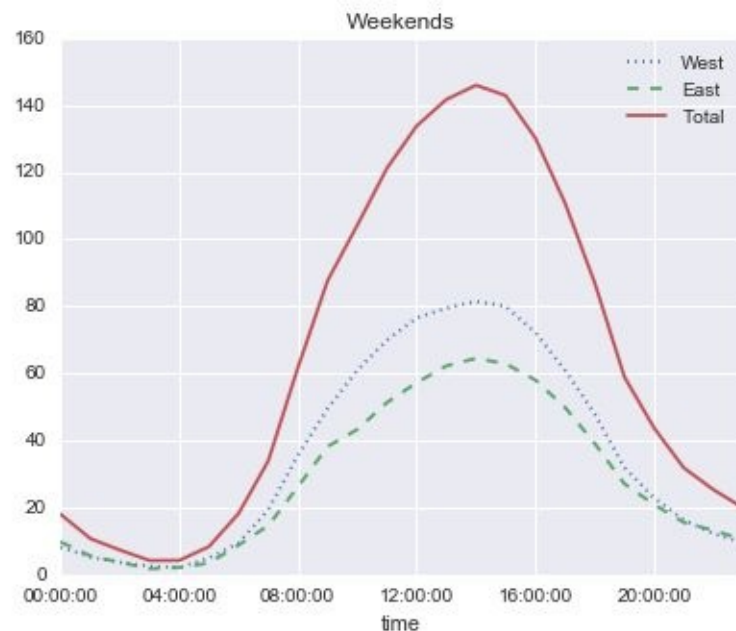
Figure 3-17. Average hourly bicycle counts by weekday and weekend
