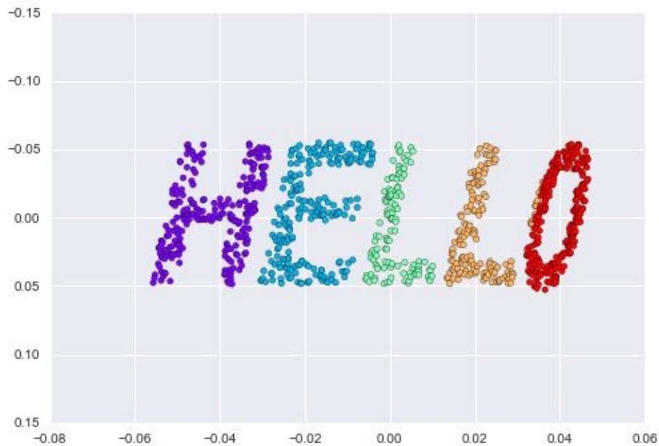
Figure 5-103. Locally linear embedding can recover the underlying data from a nonlinearly embedded input
