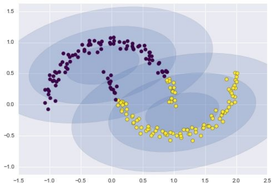
Figure 5-133. Two component GMM fit to nonlinear clusters
