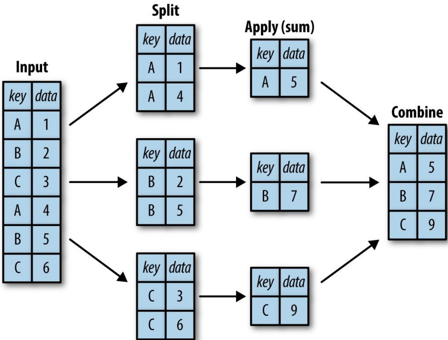
Figure 3-1. A visual representation of a groupby operation
