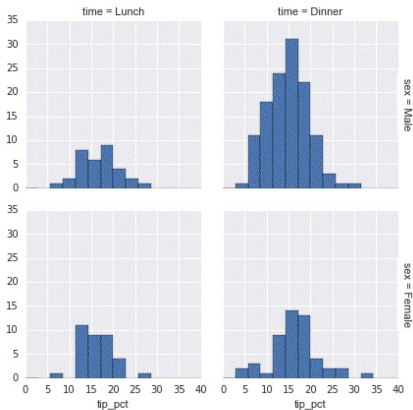
Figure 4-120. An example of a faceted histogram
