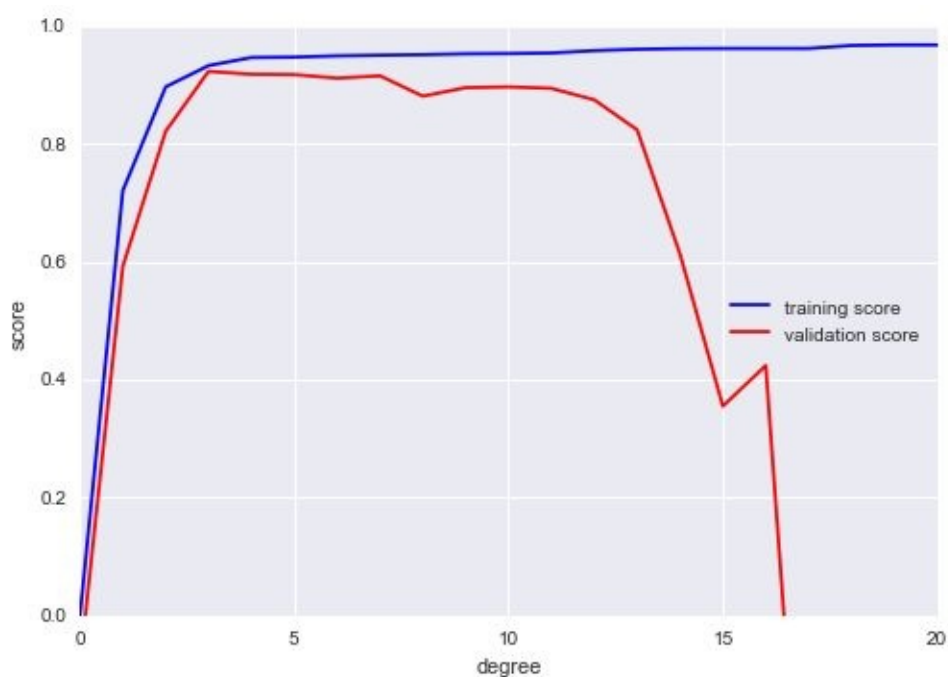
Figure 5-28. The validation curves for the data in Figure 5-27 (cf. Figure 5-26 )
