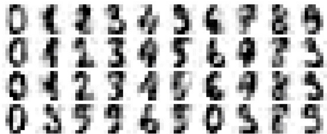
Figure 5-90. Digits “denoised” using PCA
