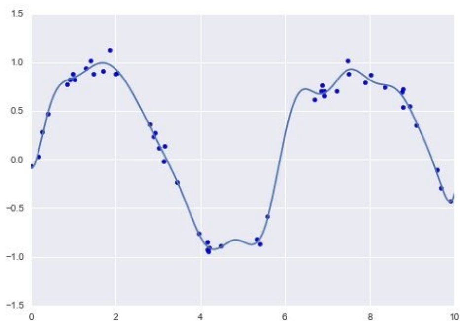
Figure 5-46. A Gaussian basis function fit computed with a custom transformer
