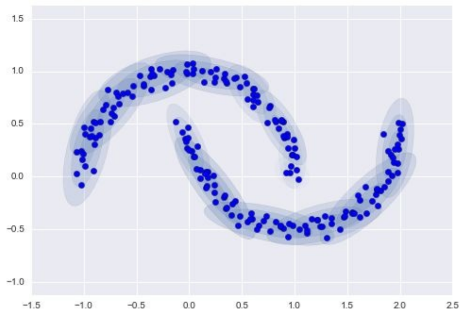
Figure 5-134. Using many GMM clusters to model the distribution of points
