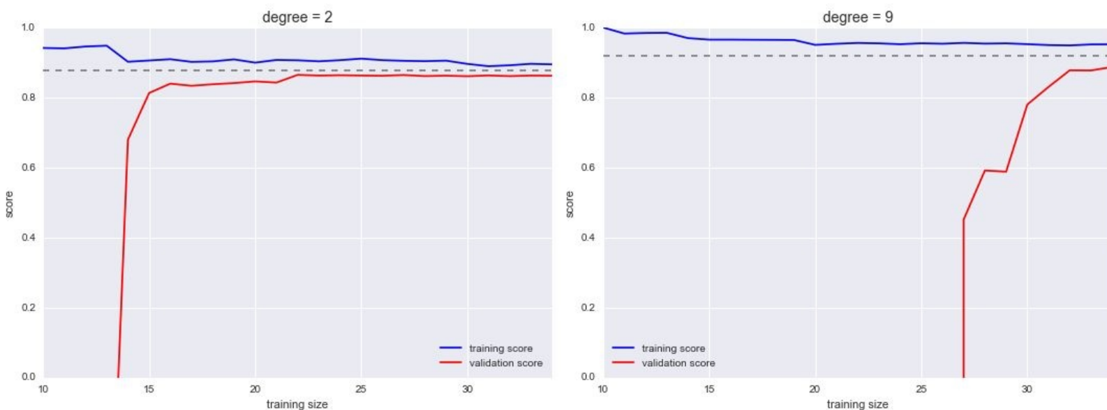
Figure 5-33. Learning curves for a low-complexity model (left) and a high-complexity model (right)
