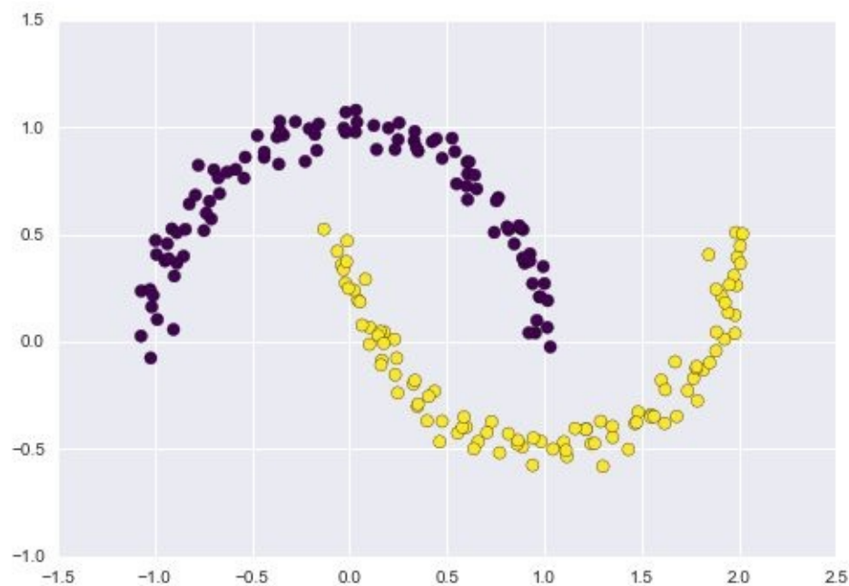
Figure 5-117. Nonlinear boundaries learned by SpectralClustering
