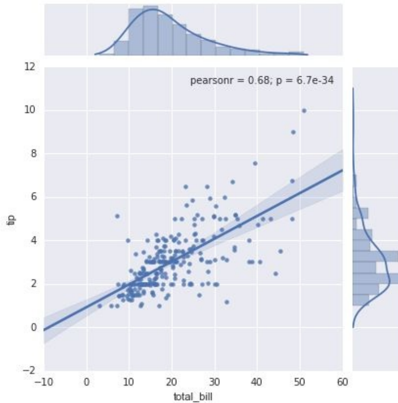
Figure 4-123. A joint distribution plot with a regression fit
