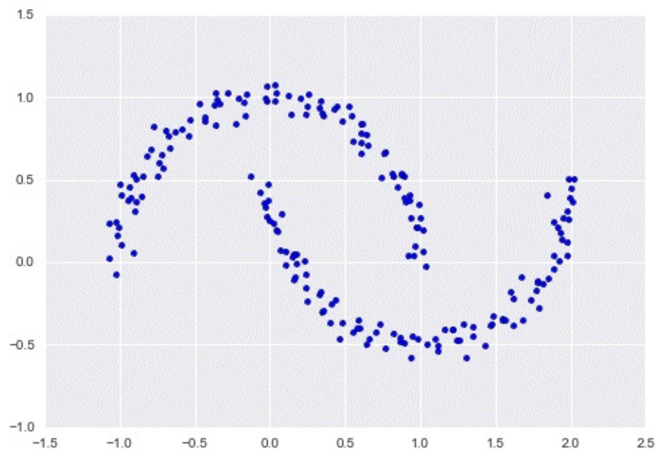
Figure 5-132. GMM applied to clusters with nonlinear boundaries
