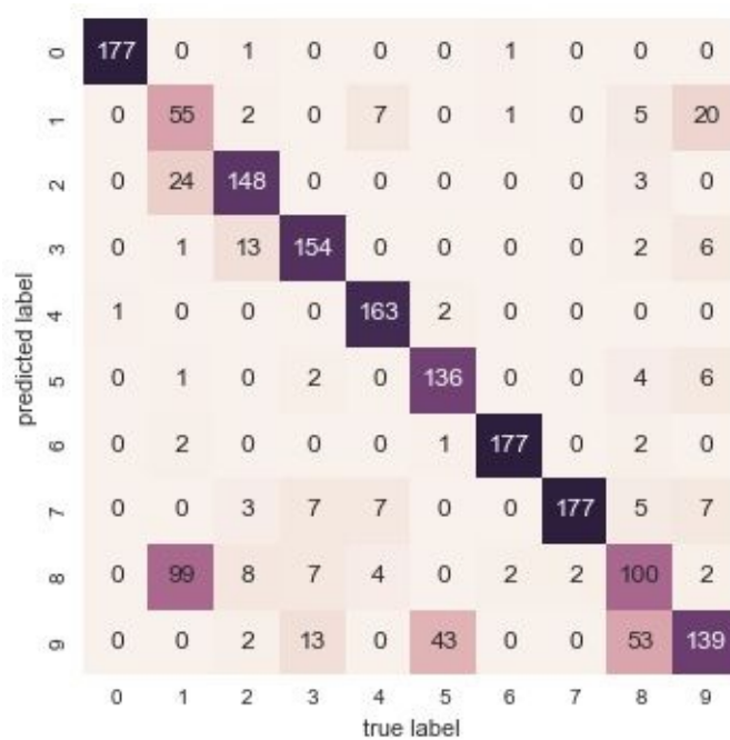
Figure 5-119. Confusion matrix for the k-means classifier
