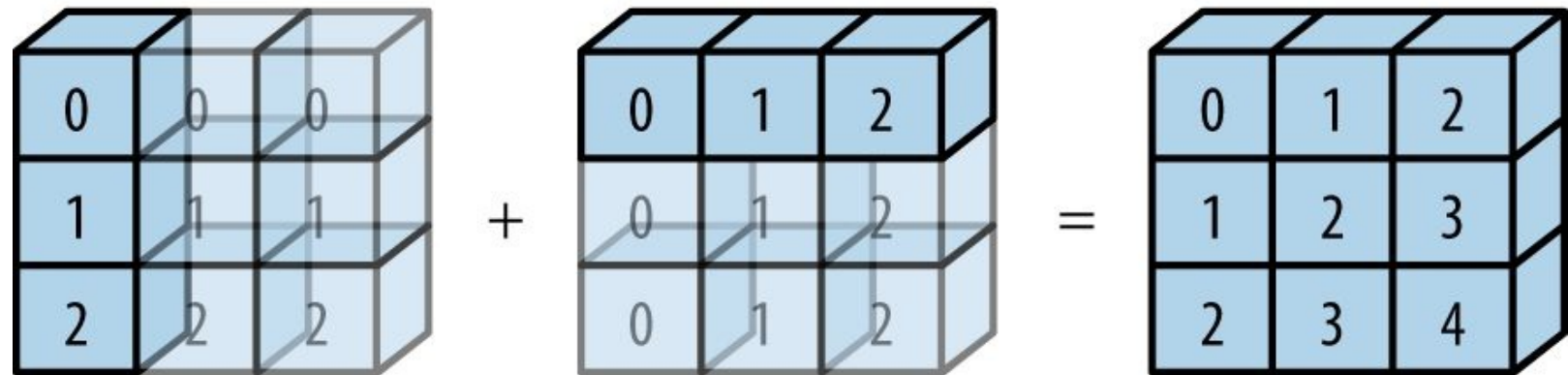
Figure 2-4. Visualization of NumPy broadcasting
