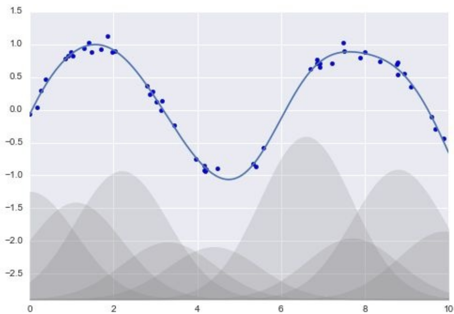
Figure 5-45. A Gaussian basis function fit to nonlinear data
