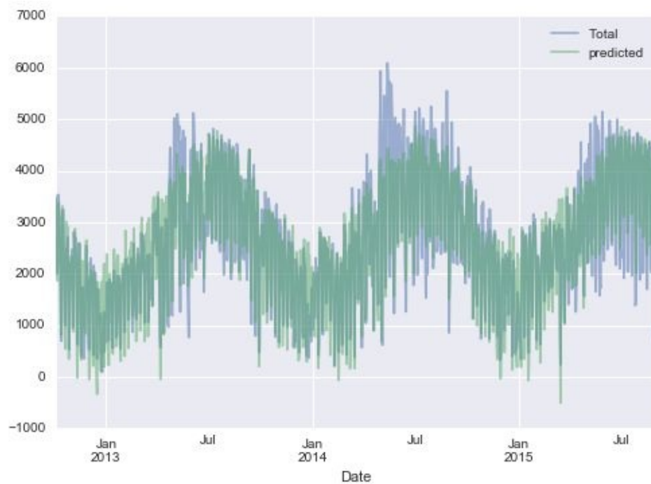
Figure 5-52. Our model's prediction of bicycle traffic
