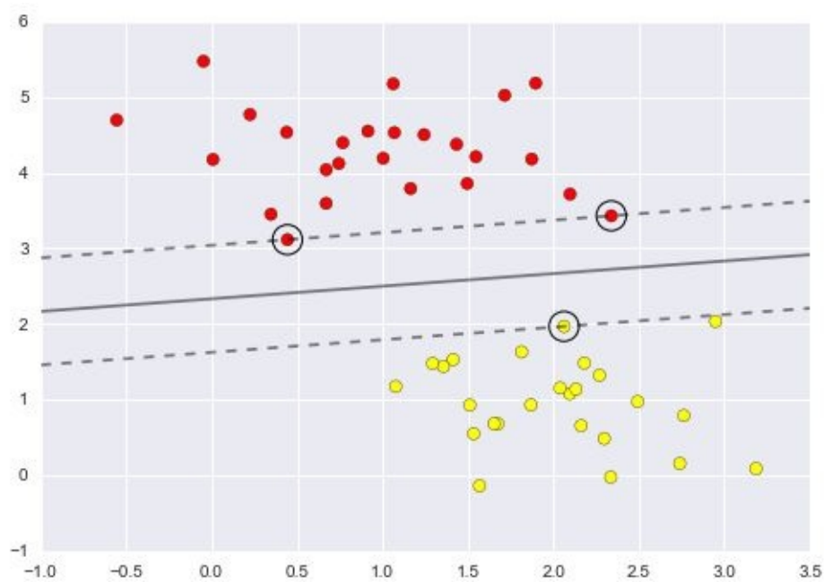
Figure 5-56. A support vector machine classifier fit to the data, with margins (dashed lines) and support vectors (circles) shown
