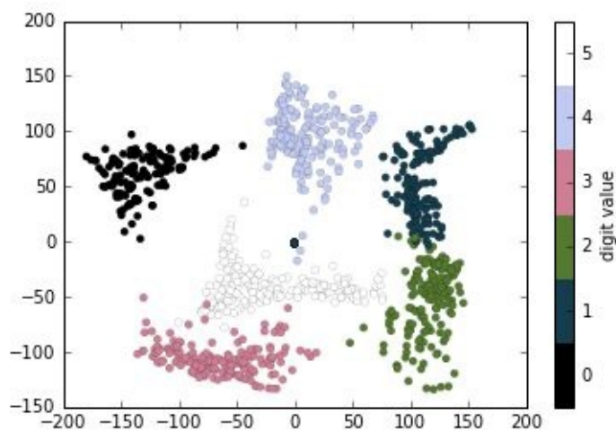
Figure 4-58. Manifold embedding of handwritten digit pixels
