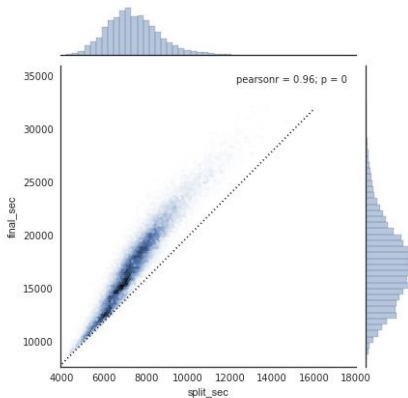
Figure 4-126. The relationship between the split for the first half-marathon and the finishing time for the full marathon
