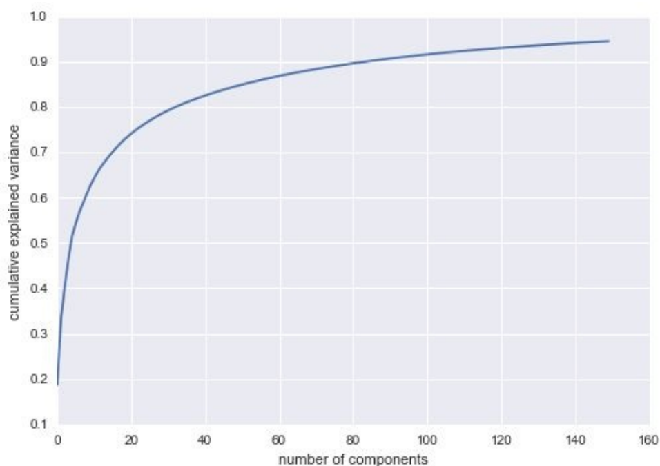
Figure 5-92. Cumulative explained variance for the LFW data
