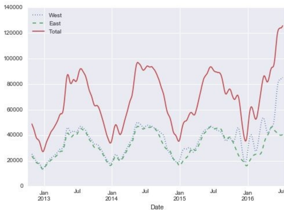
Figure 3-14. Gaussian smoothed weekly bicycle counts
