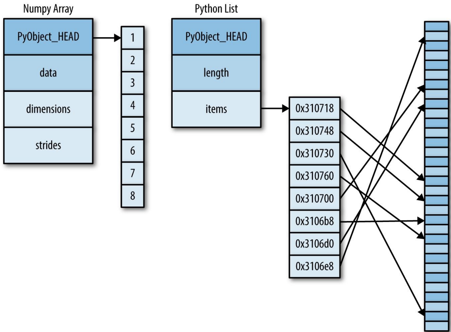
Figure 2-2. The difference between C and Python lists
