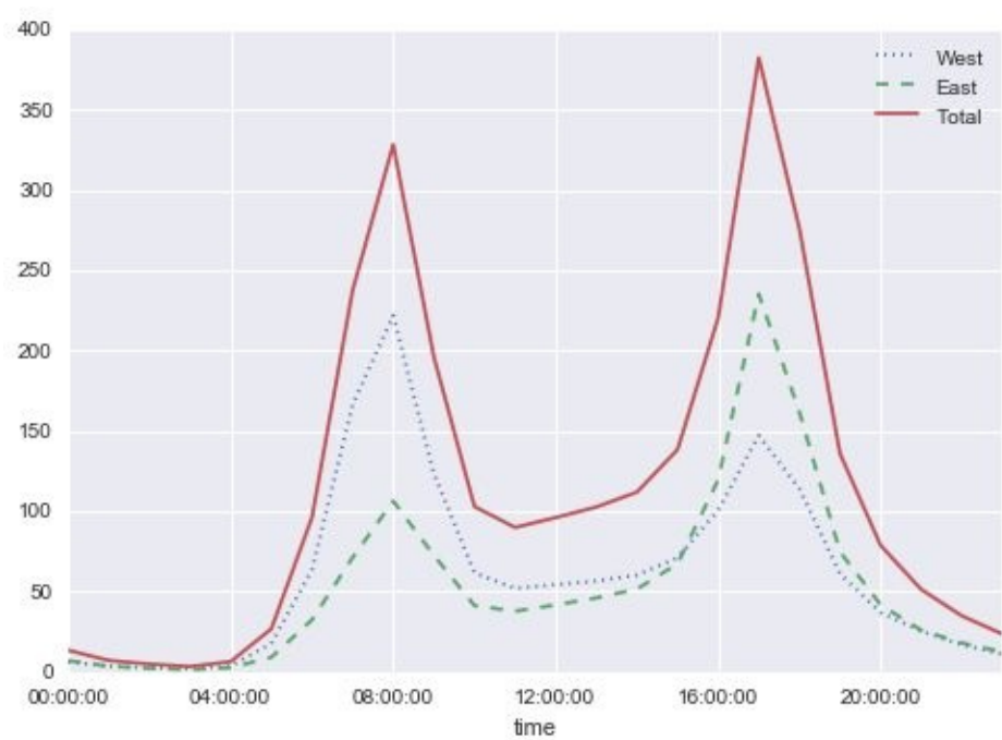
Figure 3-15. Average hourly bicycle counts
