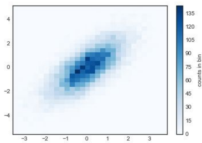
Figure 4-38. A two-dimensional histogram with plt.hist2d
