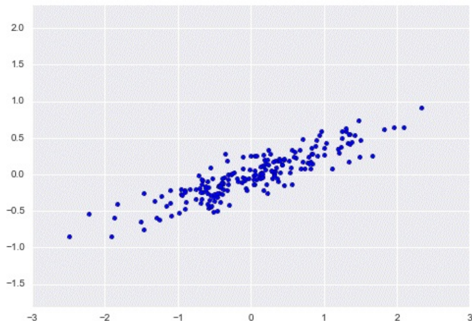
Figure 5-80. Data for demonstration of PCA
