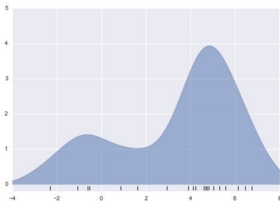
Figure 5-144. A kernel density estimate with a Gaussian kernel
