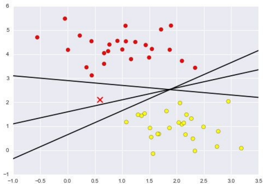
Figure 5-54. Three perfect linear discriminative classifiers for our data
