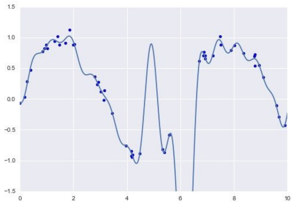
Figure 5-47. An overly complex basis function model that overfits the data
