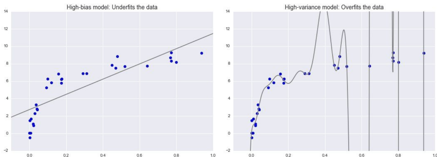
Figure 5-24. A high-bias and high-variance regression model
