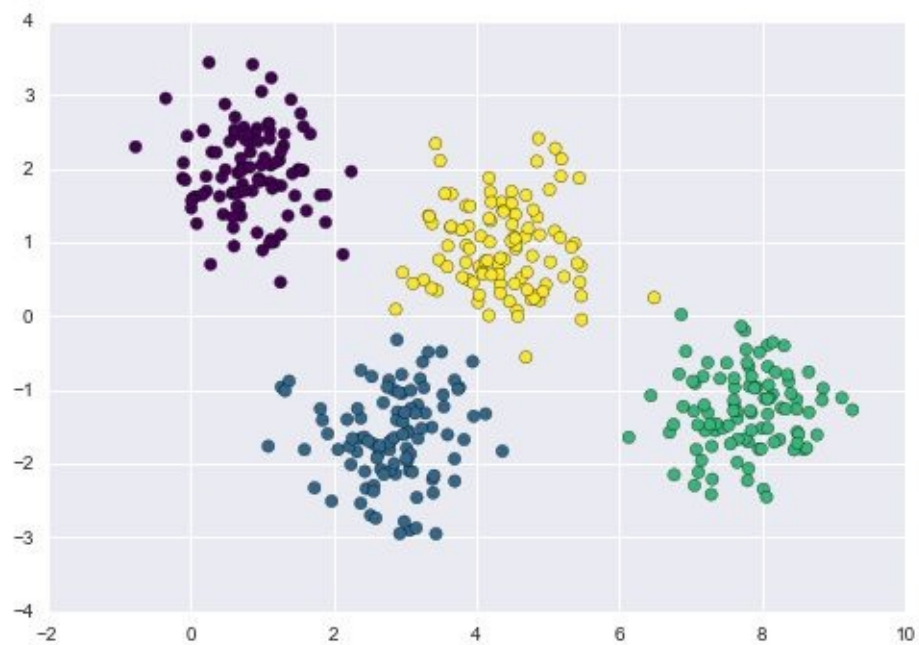
Figure 5-127. Gaussian mixture model labels for the data
