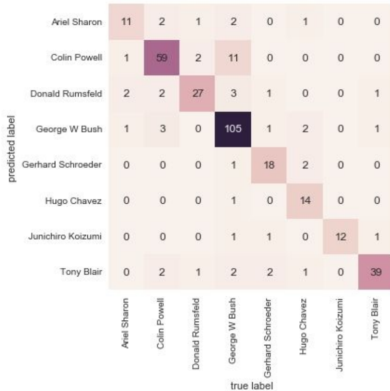
Figure 5-66. Confusion matrix for the faces data
