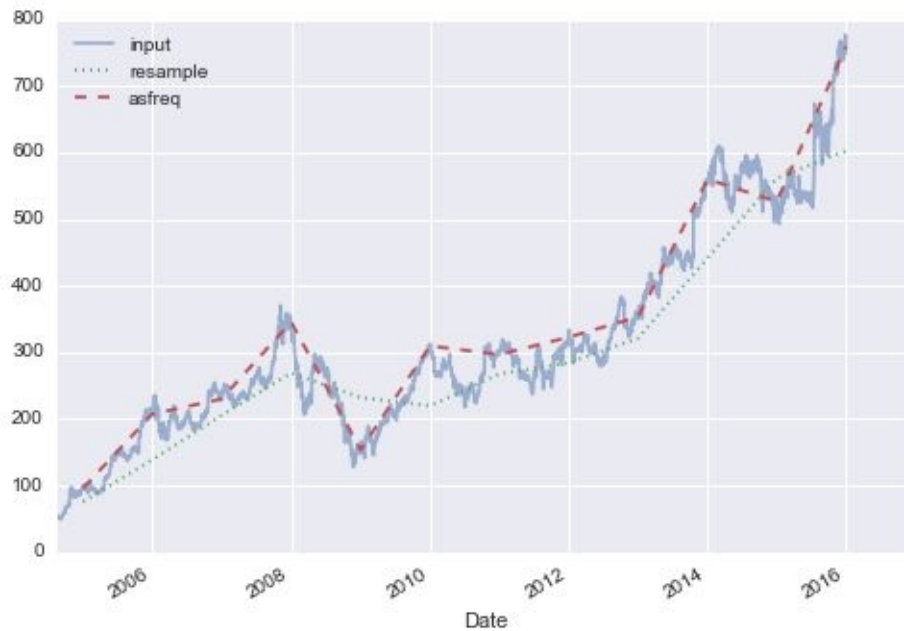
Figure 3-6. Resamplings of Google's stock price
