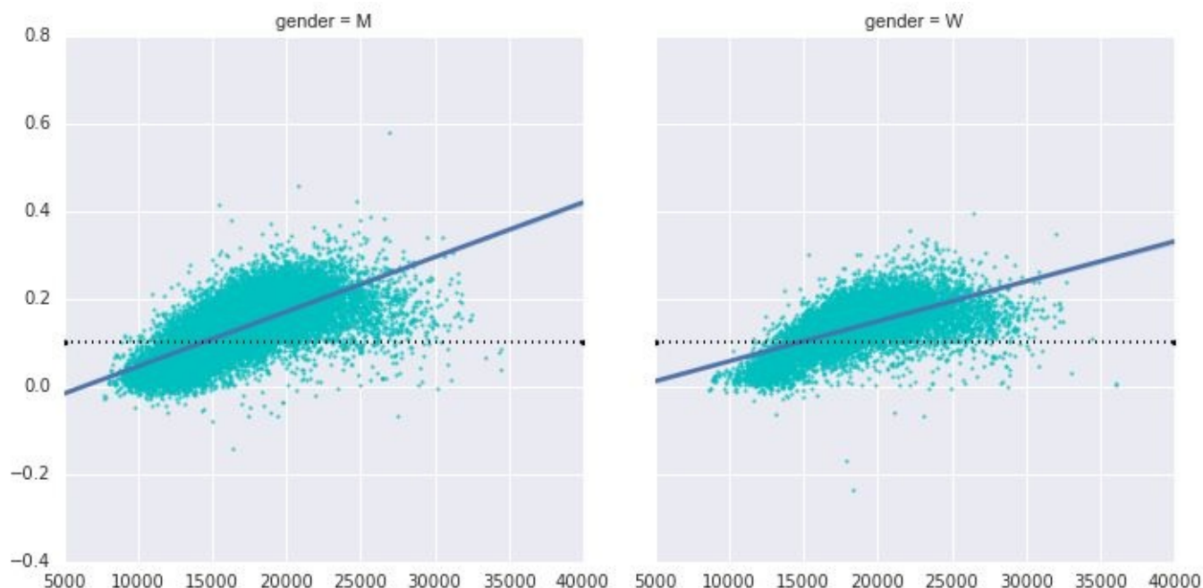
Figure 4-132. Split fraction versus finishing time by gender
