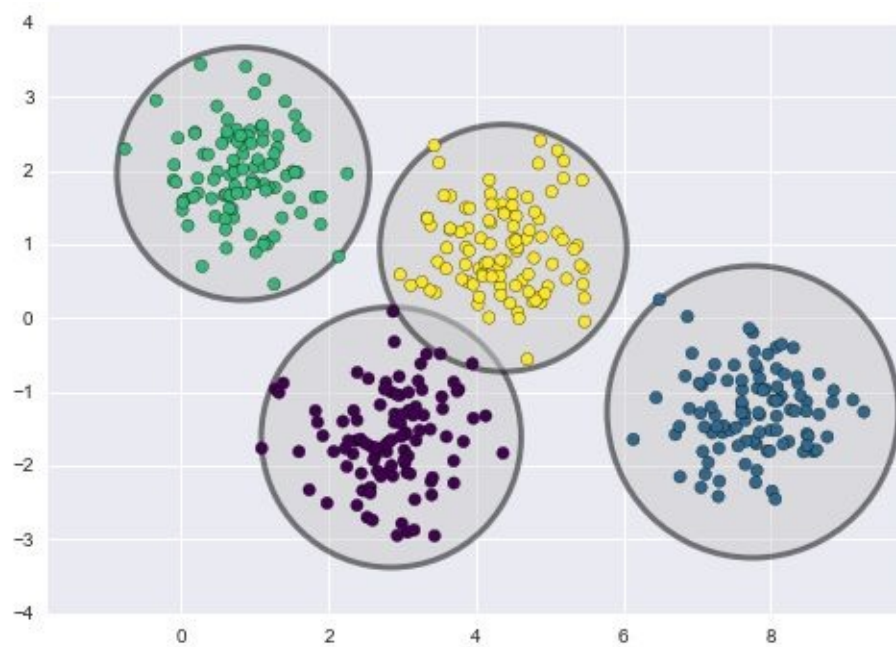
Figure 5-125. The circular clusters implied by the k -means model
