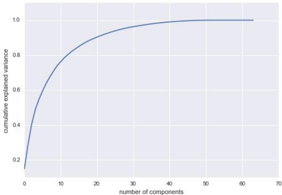
Figure 5-87. The cumulative explained variance, which measures how well PCA preserves the content of the data
