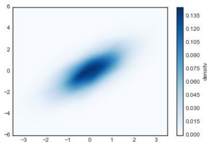
Figure 4-40. A kernel density representation of a distribution
