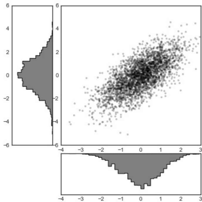
Figure 4-66. Visualizing multidimensional distributions with plt.GridSpec
