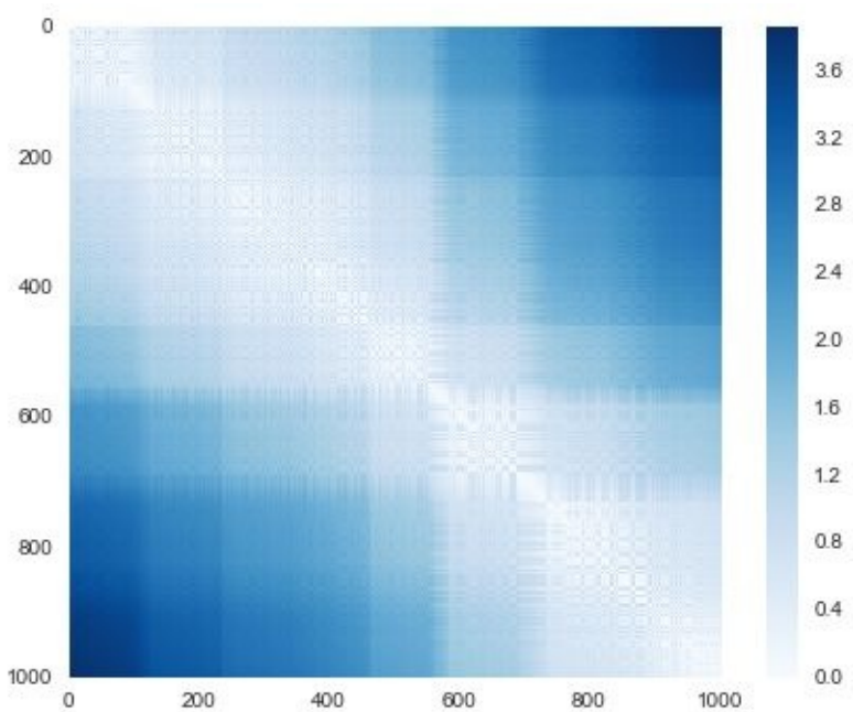
Figure 5-96. Visualization of the pairwise distances between points
