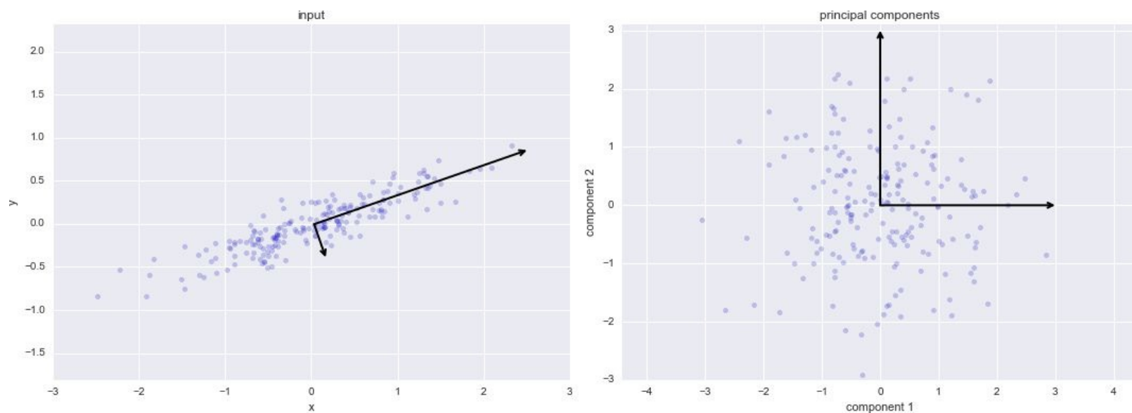
Figure 5-82. Transformed principal axes in the data
