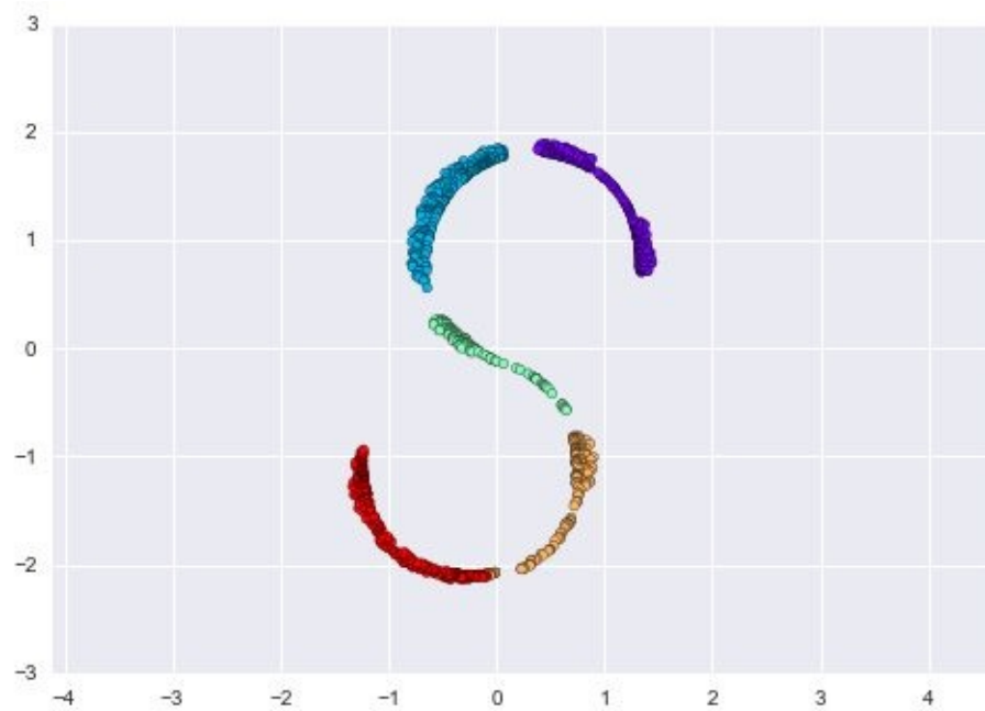
Figure 5-101. The MDS algorithm applied to the nonlinear data; it fails to recover the underlying structure
