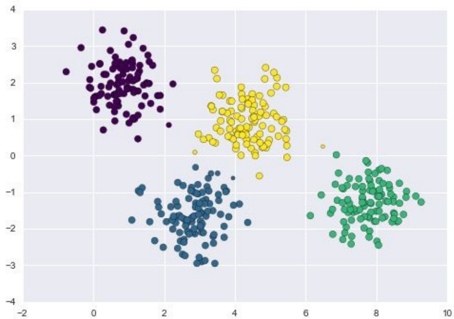
Figure 5-128. GMM probabilistic labels: probabilities are shown by the size of points
