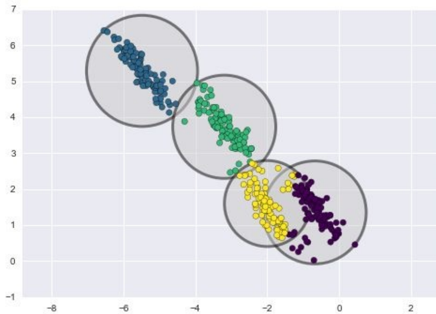
Figure 5-126. Poor performance of k -means for noncircular clusters
