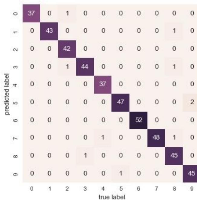
Figure 5-79. Confusion matrix for digit classification with random forests
