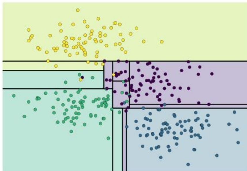
Figure 5-71. First frame of the interactive decision tree widget; for the full version, see the online appendix
