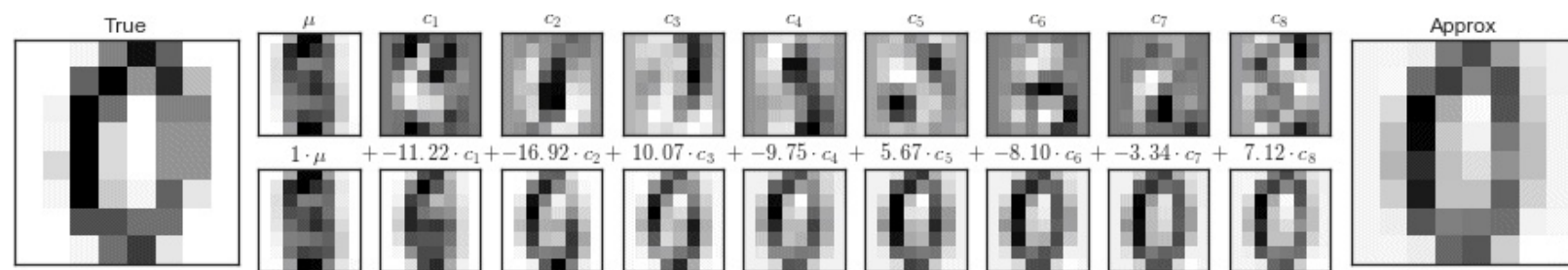
Figure 5-86. A more sophisticated dimensionality reduction achieved by discarding the least important principal components (compare to Figure 5-85 )
