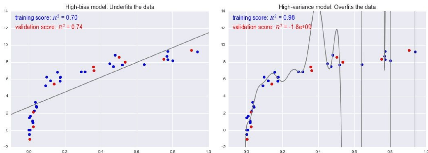
Figure 5-25. Training and validation scores in high-bias and high-variance models
